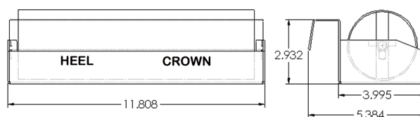
511 - Top Mounting Bun Dresser (Manual Only)
